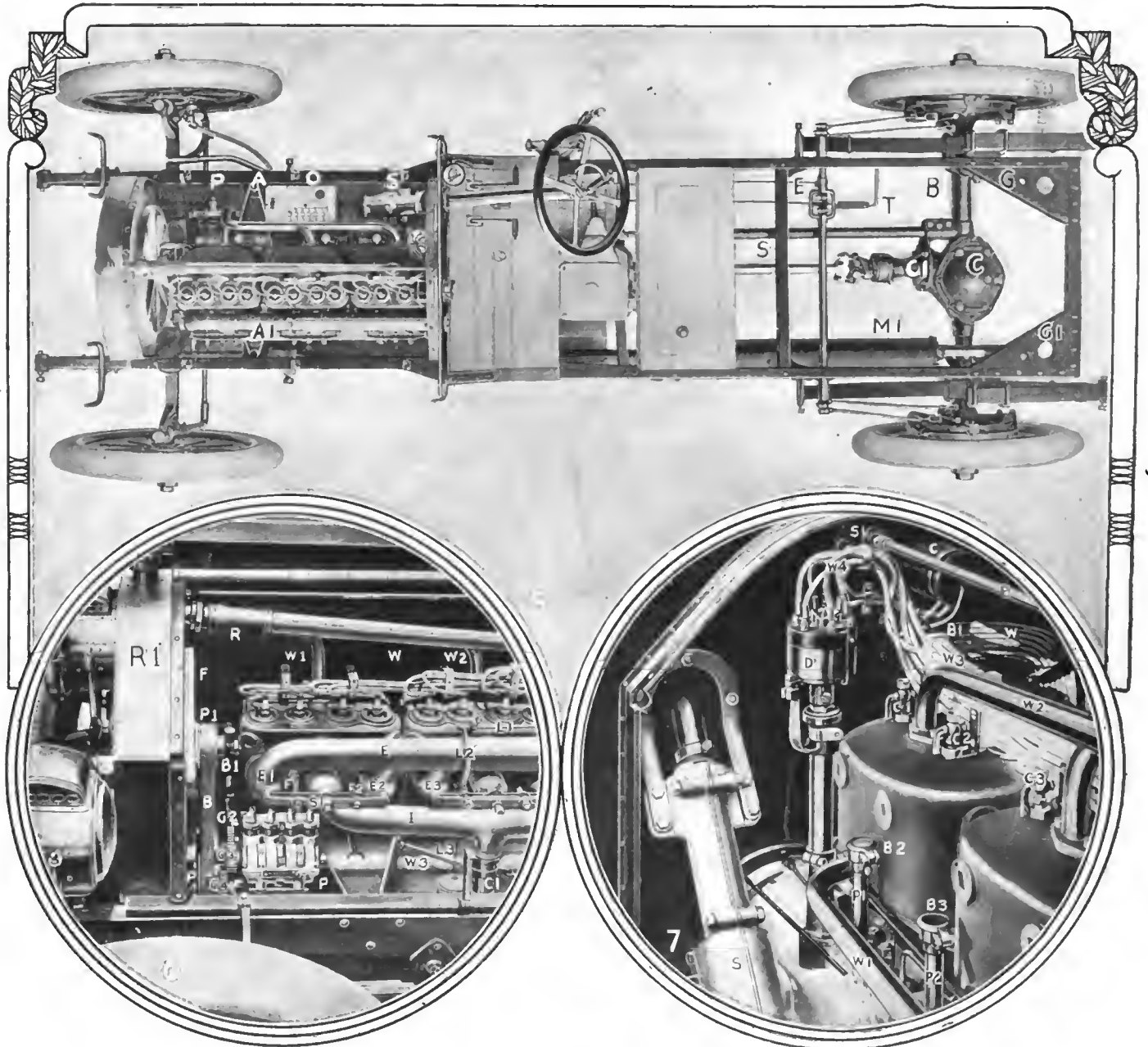
Fig. 5—Plan view of the model AA chassis showing the six-cylinder motor and the live rear axle. Fig. 6—Front end of the motor showing tire inflation pump. Fig. 7—Right-hand side of motor, showing distributor and coil on the dash
